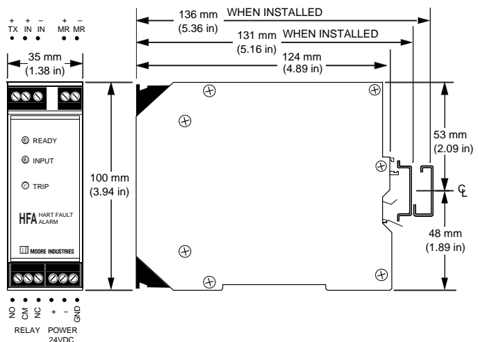
Figure 2. HFA Dimensions
