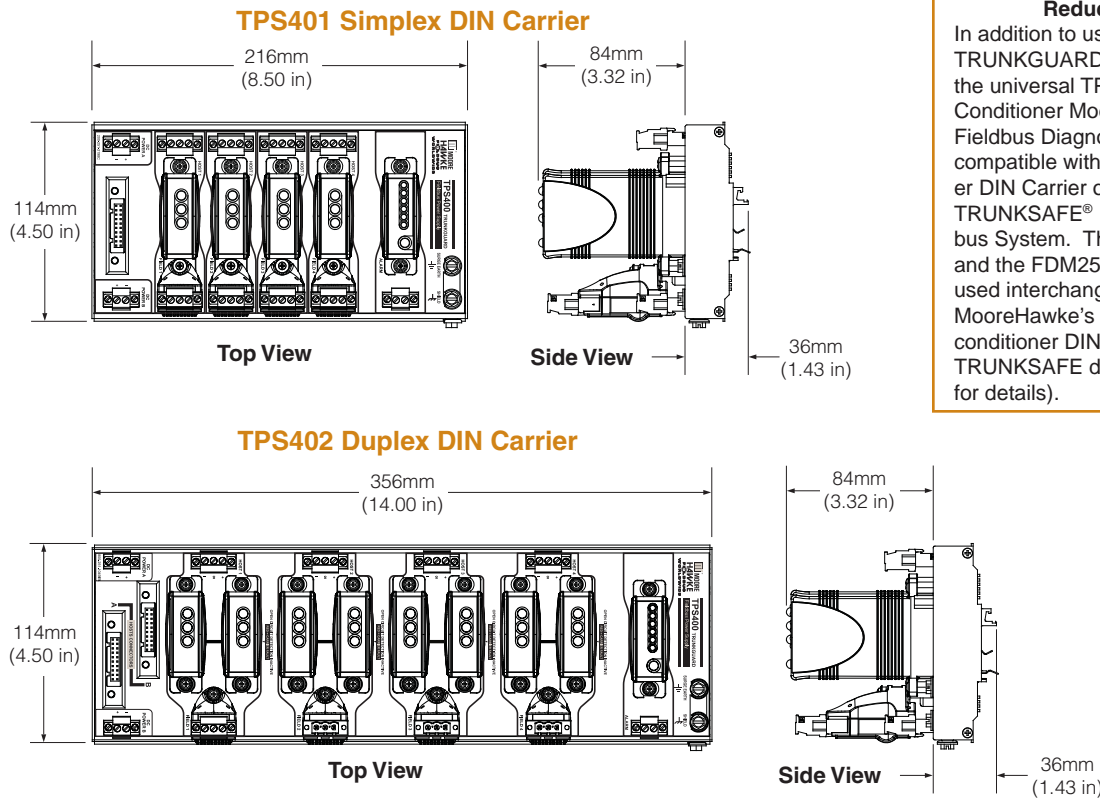
Figure 3. Installation Dimensions.
