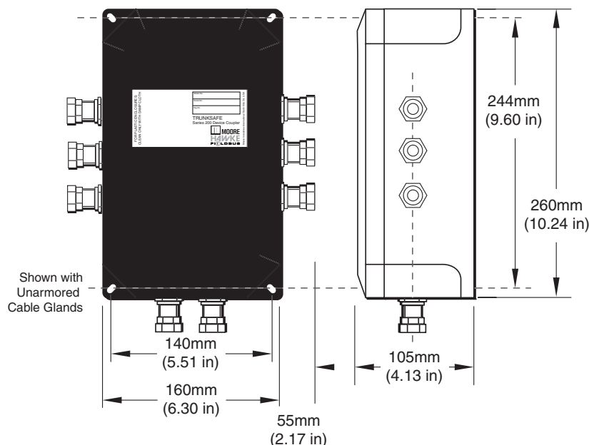
Figure 6. GRP (Glass Reinforced Polyester) Enclosure Installation Dimensions for 6-Spur (TS236) Models.
