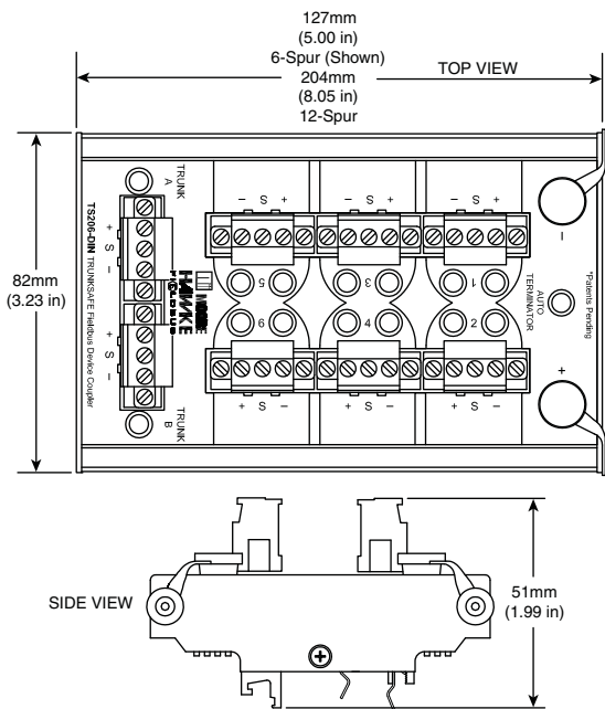
Figure 3. TS200 Device Coupler DIN-Rail Mounting Installation Dimensions (Base Unit).
