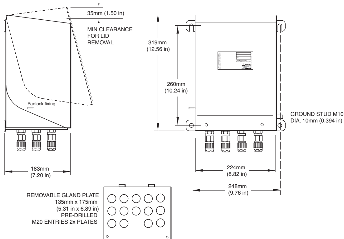
Figure 6. GRP (Glass Reinforced Polyester) Enclosure Installation Dimensions for 6-Spur (TS236) Models.
