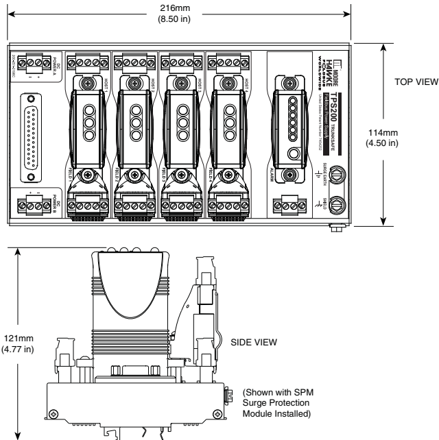
Figure 2. TPS201/202 Advanced Power Conditioner with DIN-Rail Mounting Installation Dimensions.
