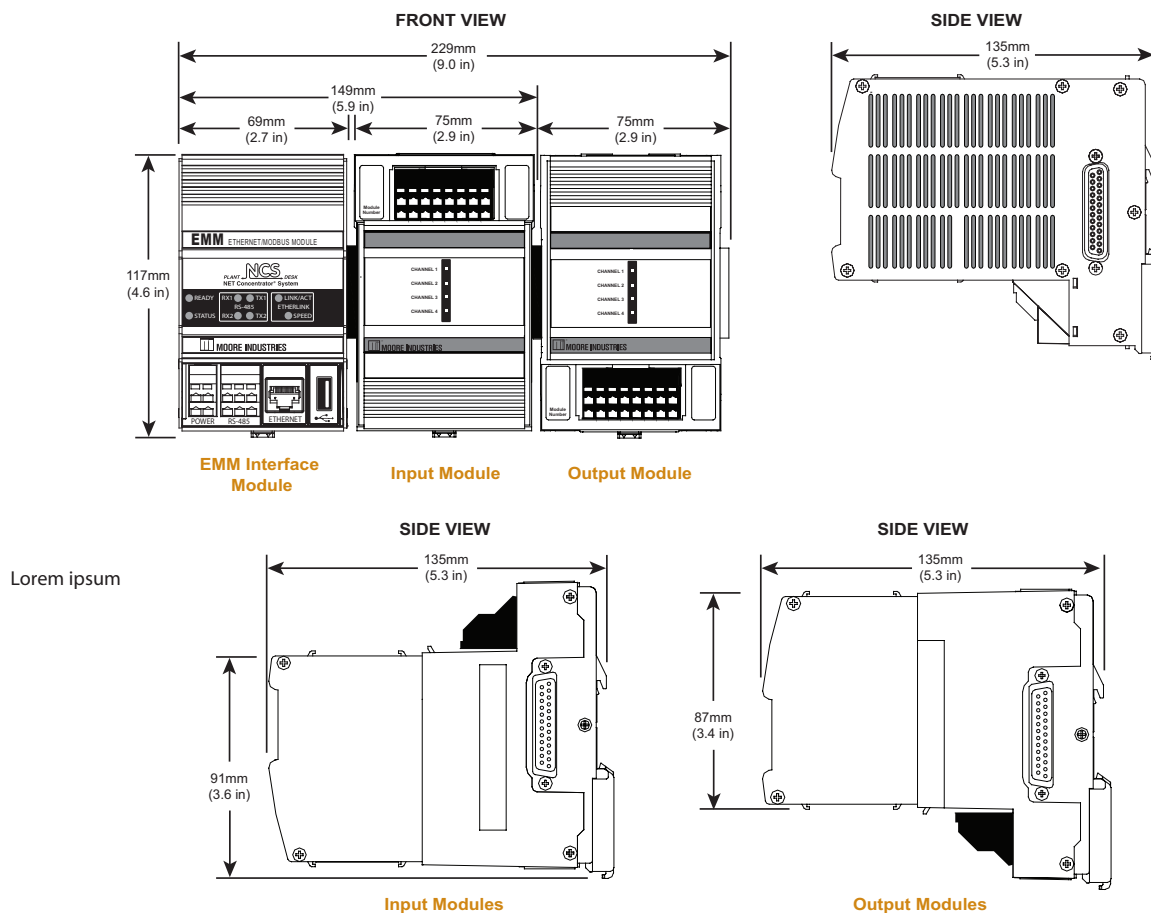
Figure 9. Installation Dimensions.
